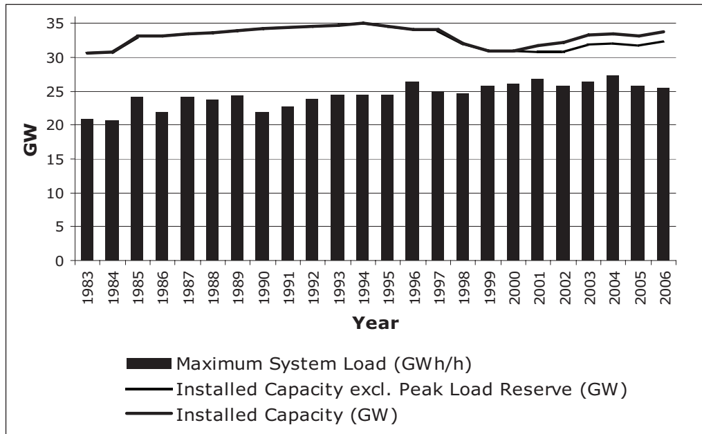
Figure 3.1 Installed capacity and System Load in Sweden 1983-2006
